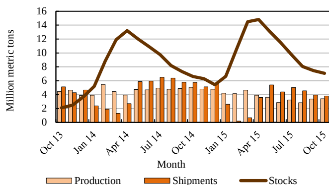
Figure 1. Monthly domestic production, shipments, and stocks of iron ore from October 2013–October 2015. Source: U.S. Geological Survey
